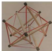
Tensegrity-Modell
